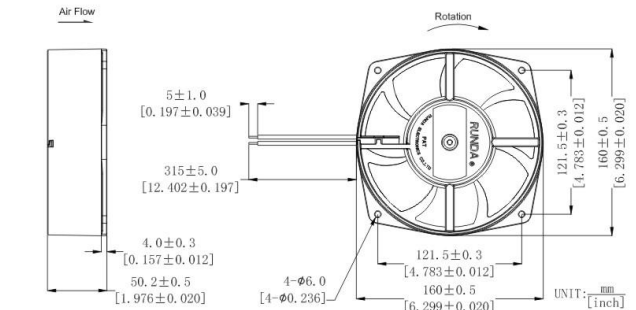
DIMENSIONS DRAWING
