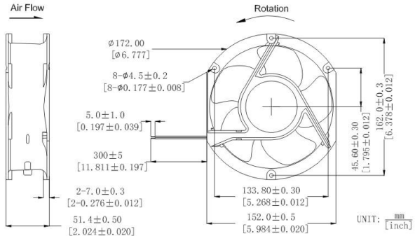
DIMENSIONS DRAWING
