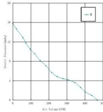
Fan Performance Curve
