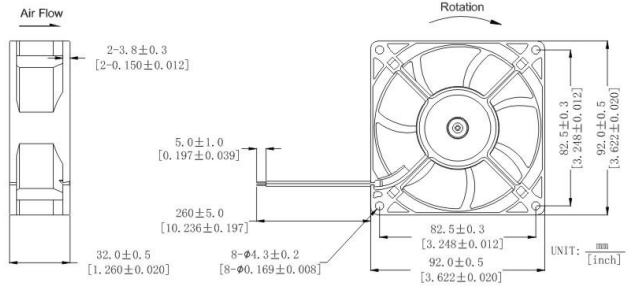
DIMENSIONS DRAWING
