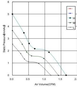
Fan Performance Curve
