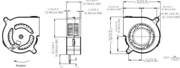
DIMENSIONS DRAWING
