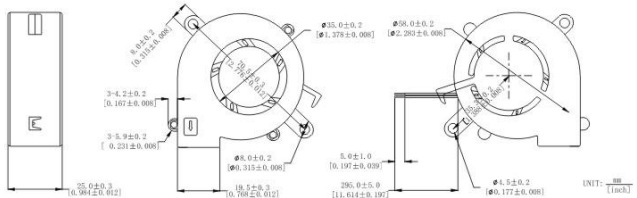
DIMENSIONS DRAWING
