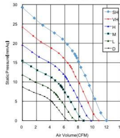
Fan Performance Curve
