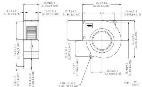
DIMENSIONS DRAWING
