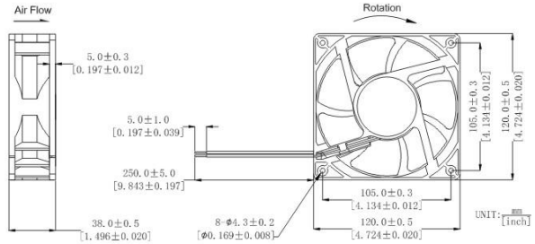
DIMENSIONS DRAWING
