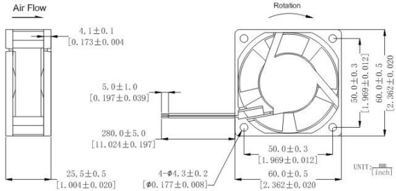
DIMENSIONS DRAWING
