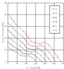
Fan Performance Curve
