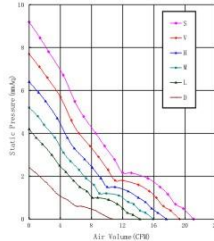
Fan Performance Curve
