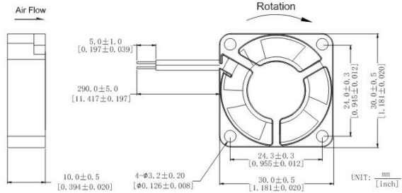
DIMENSIONS DRAWING
