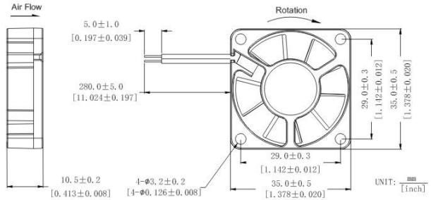
DIMENSIONS DRAWING
