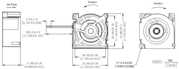
DIMENSIONS DRAWING
