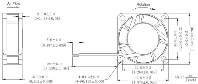
DIMENSIONS DRAWING
