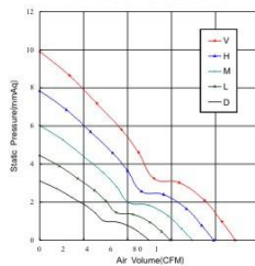
Fan Performance Curve
