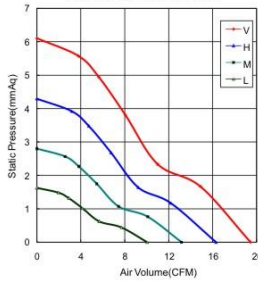
Fan Performance Curve
