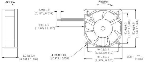
DIMENSIONS DRAWING
