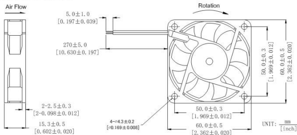
DIMENSIONS DRAWING
