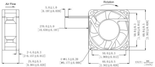
DIMENSIONS DRAWING
