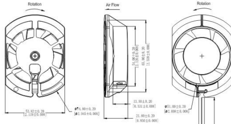
DIMENSIONS DRAWING
