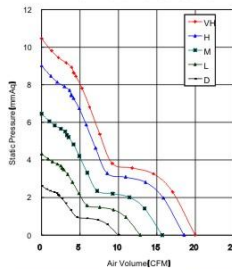
Fan Performance Curve
