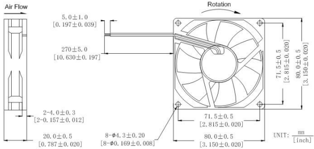
DIMENSIONS DRAWING
