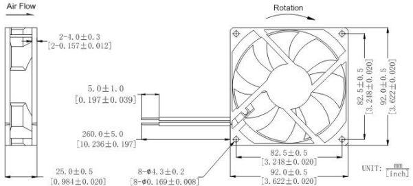
DIMENSIONS DRAWING
